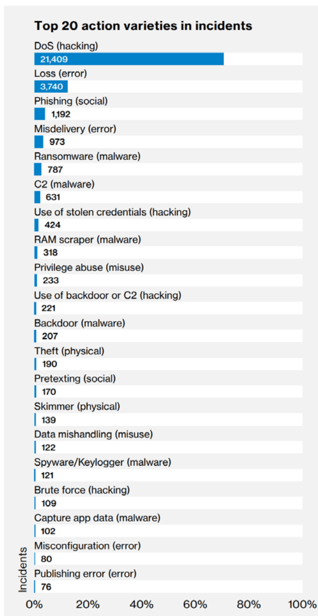
Figure 4. Top 20 threat action varieties (incidents) (n=30,362)
